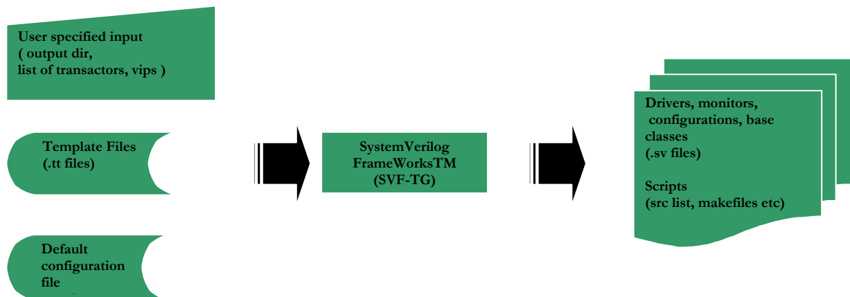
Figure 1. SystemVerilog FrameWorks™ (SVF-TG) tool
